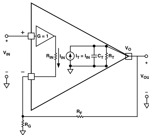
Figure 5. Model of Current Feedback Amplifier
